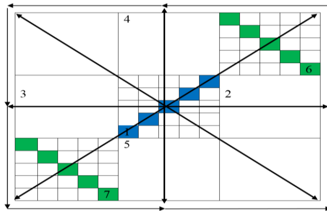
Figure 7. The base according to the pattern is a pattern drawn on the diagonal axis passing the center of the coil axis of 1/4 wrap.
